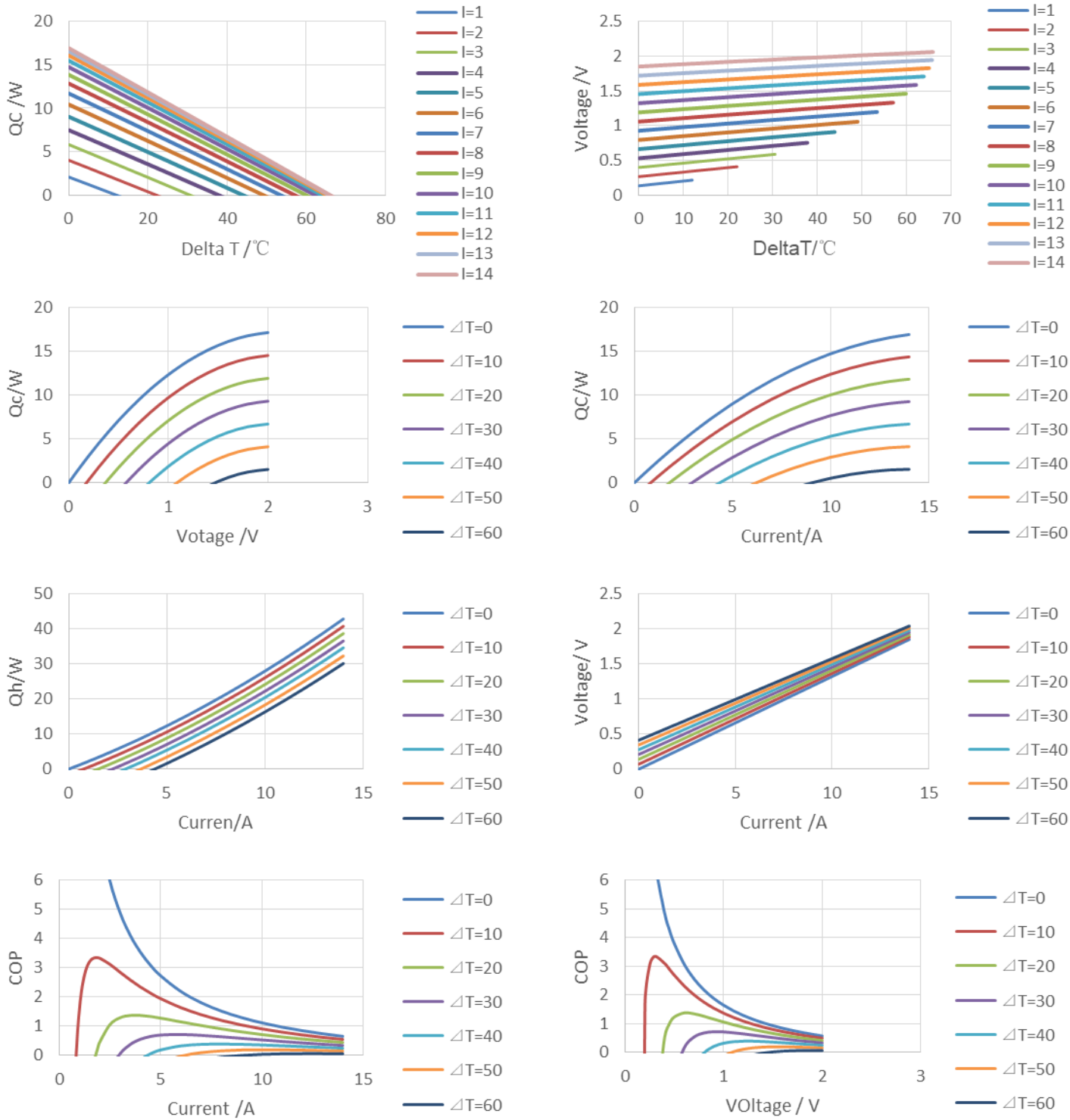
Performance Curves at T_h=27\text{ }^\circ\text{C}
