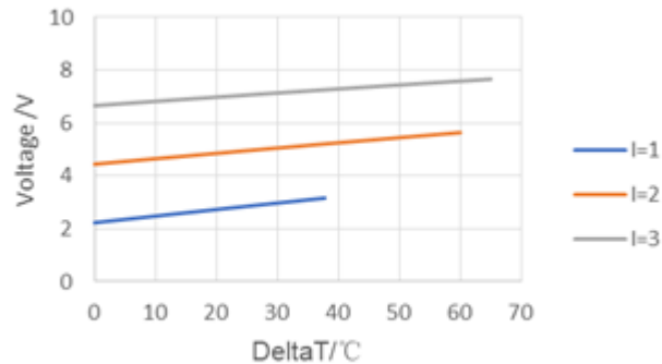
Performance Curves at Th=27 °C
