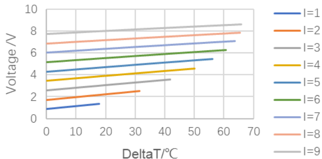
Performance Curves at T_h=27\text{ }^\circ\text{C}
