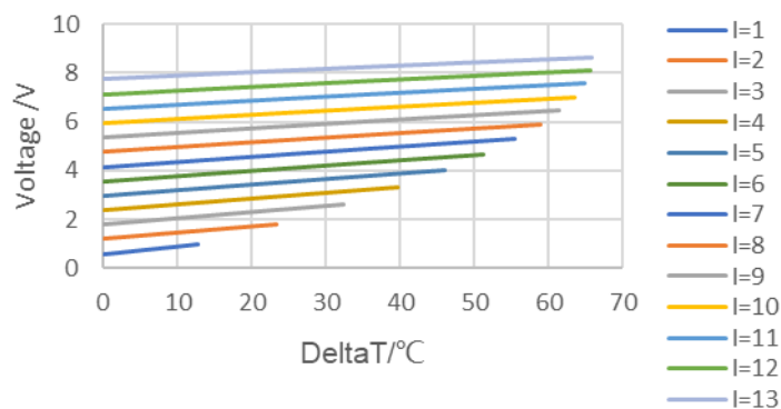
Performance Curves at T_h = 27^\circ\text{C}
