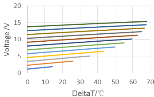
Performance Curves at T_h=27^\circ\text{C}
