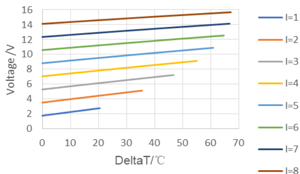
Performance Curves at T_h=27\text{ }^\circ\text{C}
