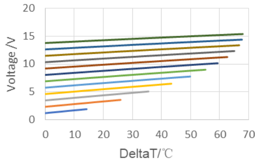
Performance Curves at Th=27 °C
