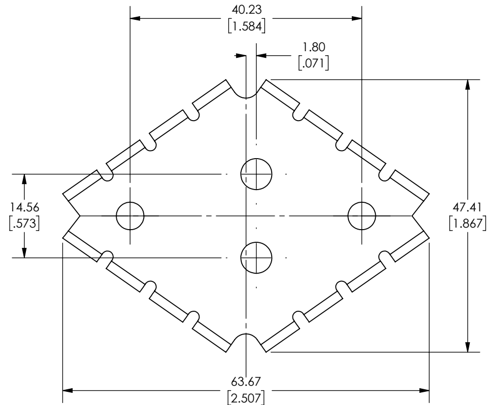
Top View Scale 3:2
