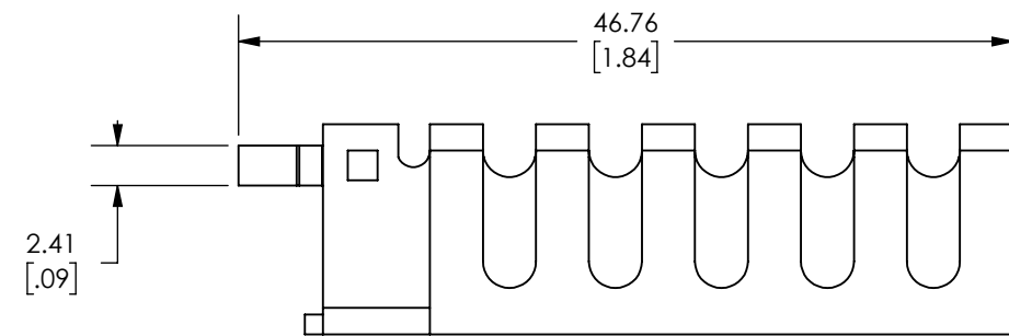
Side View
