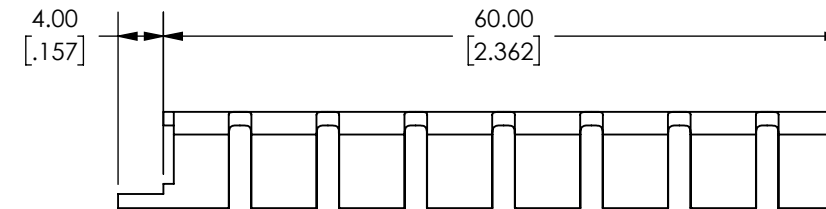
Side View Scale 3:2
