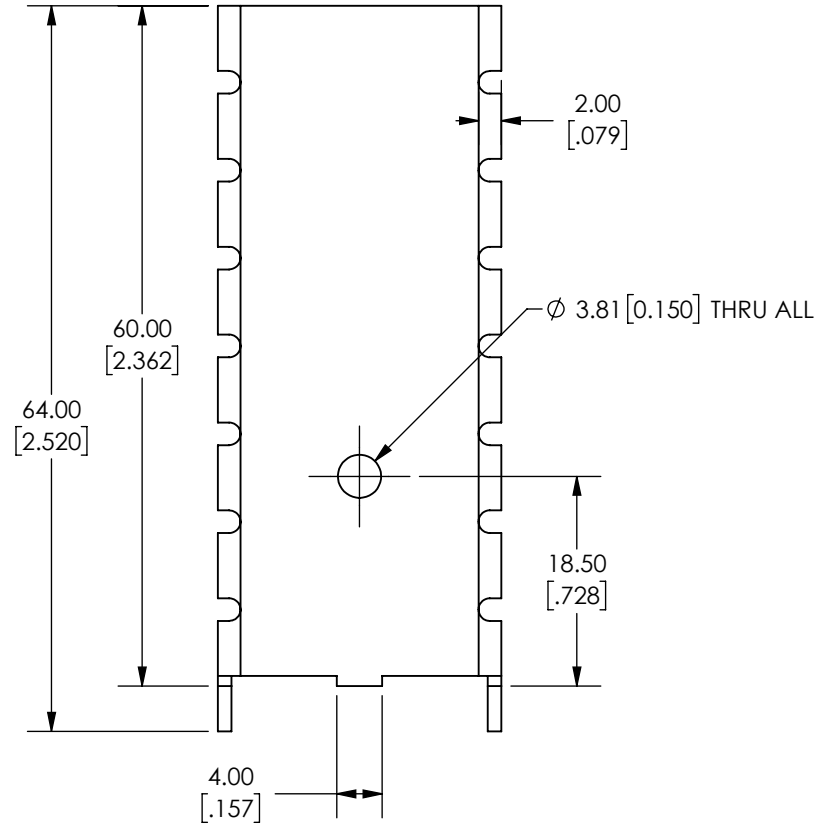
Top View Scale 3:2
