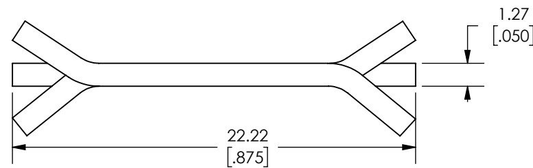
Bottom View Scale 7:2
