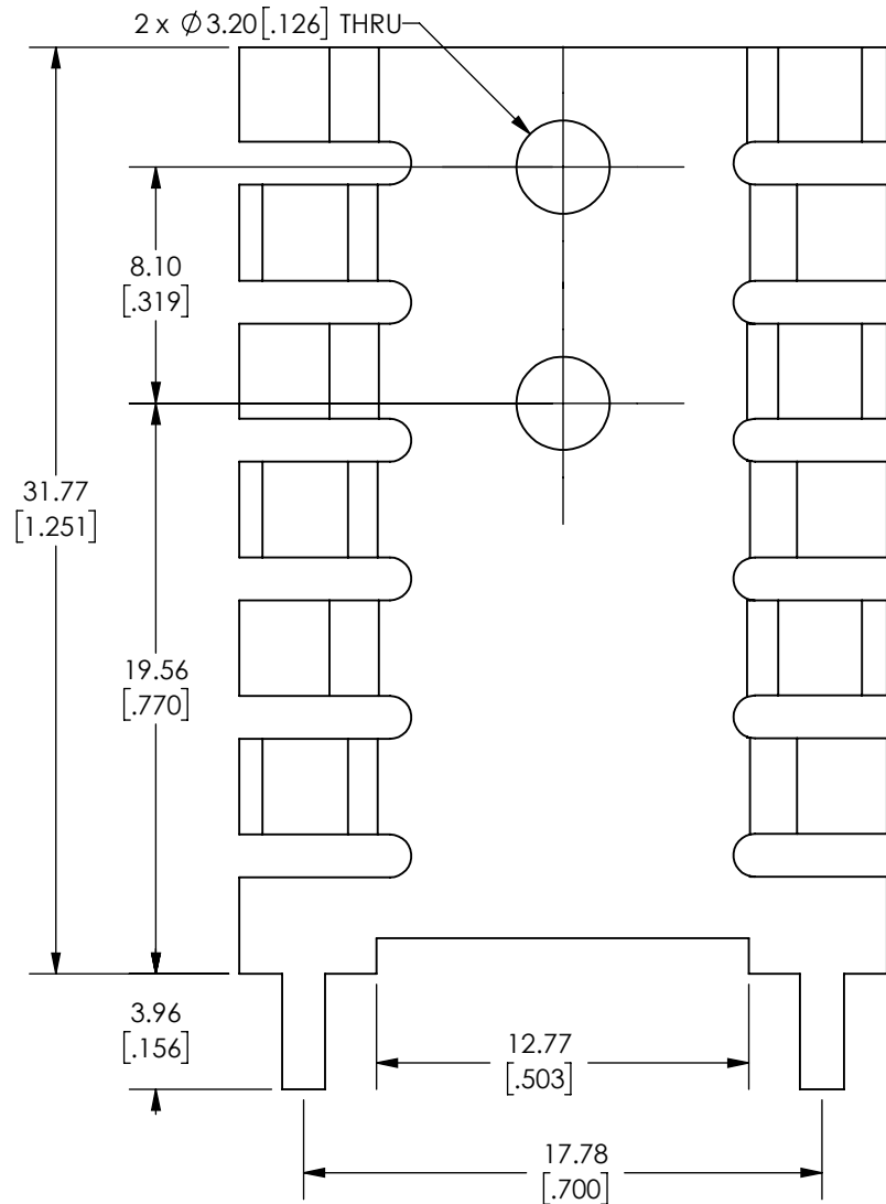
Front View Scale 7:2
