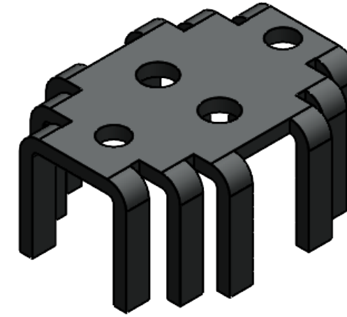
Isometric View NTS
