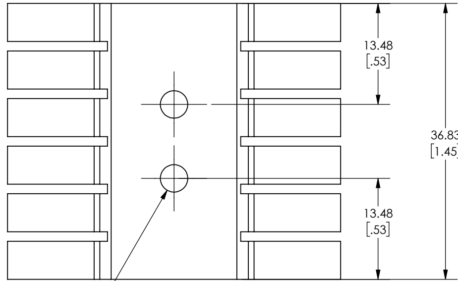
2X \varnothing 3.66[0.14] THRU ALL Top View Scale 2:1
