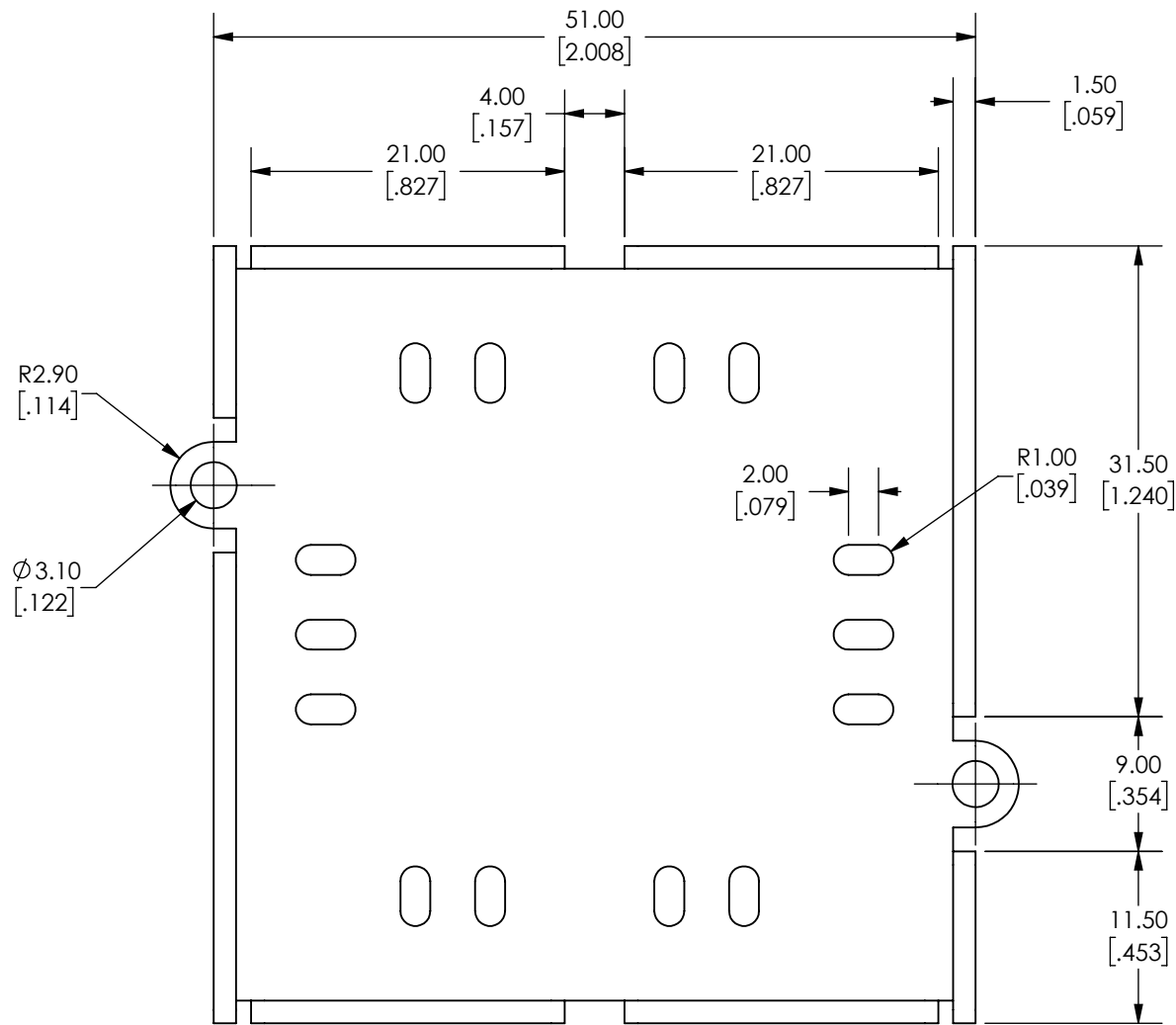
Front View
