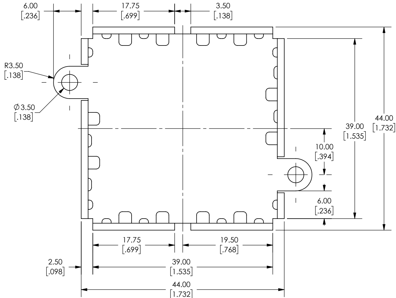
Top View Scale 2:1
