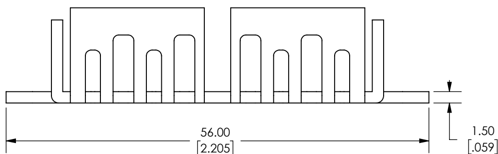
Front View Scale 2:1
