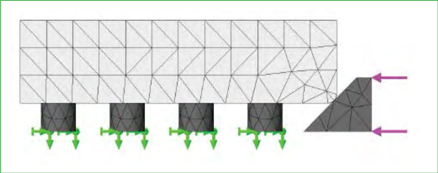
Figure 3. Model of BGA Component with Frame Clip (FC) Wedge Interaction.
