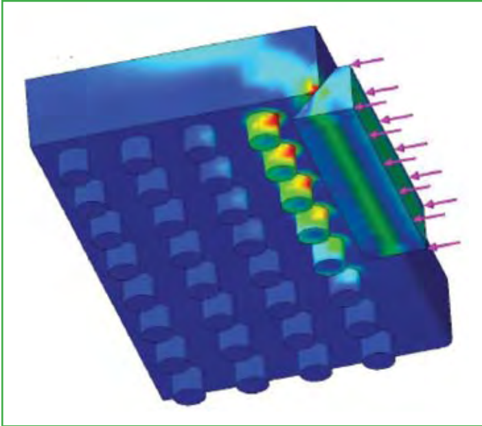
Figure 4. von Mises Stress Plot for BGA with maxiGRIP™ Frame Clip Installed.
