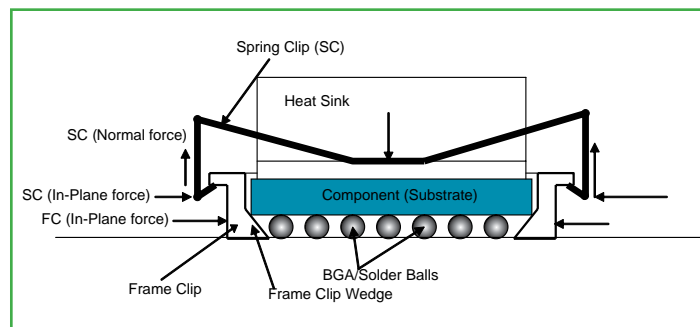
Figure 2. Cutaway of BGA Component with maxiGRIP Heat Sink Attachment.
