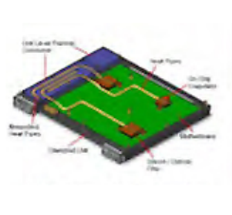
d) On board heat pipes by McGlen et al. 4
