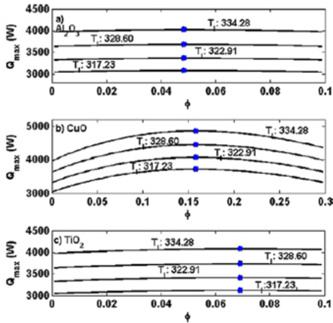
Figure 3. Maximum Heat Transfer Limit of Heat Pipes with Various Nanofluids [5]
